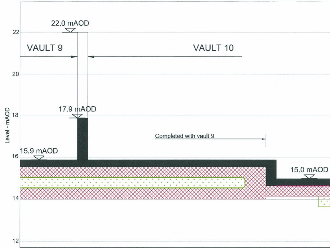
SECTION BETWEEN VAULTS 9 AND 10
