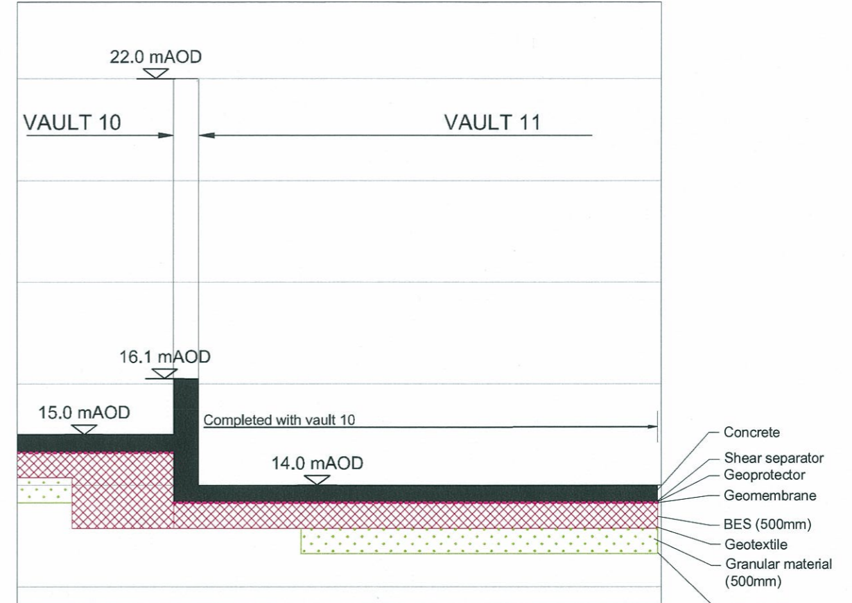
SECTION BETWEEN VAULTS 10 AND 11
